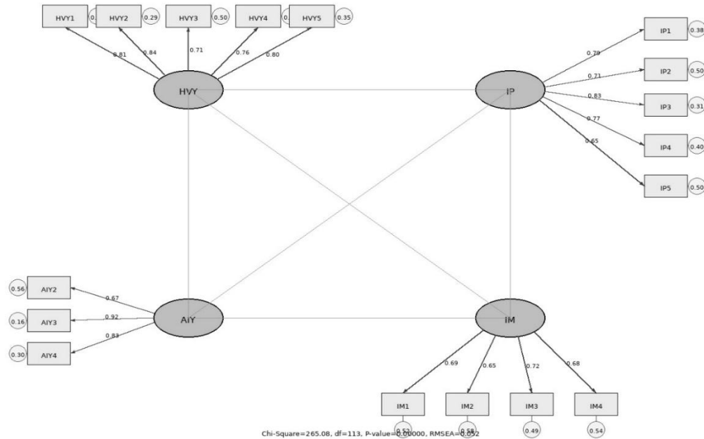
Figure 2 Confirmatory factor analysis model
